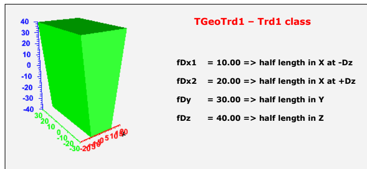
Figure 19-4 TGeoTrd1 class
