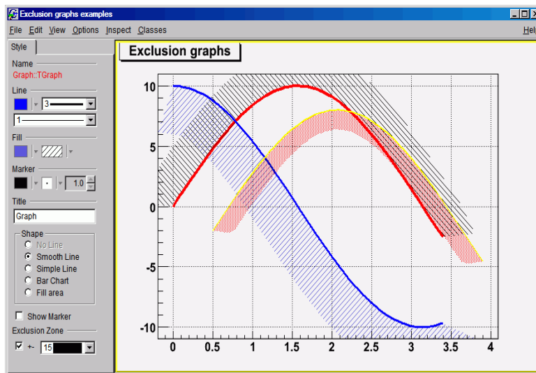
Figure 4-9 Graphs with exclusion zones
