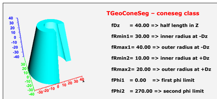
Figure 19-15 TGeoConeSeg Class
