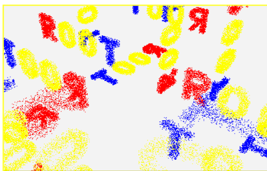
Figure 19-32 Random rays
