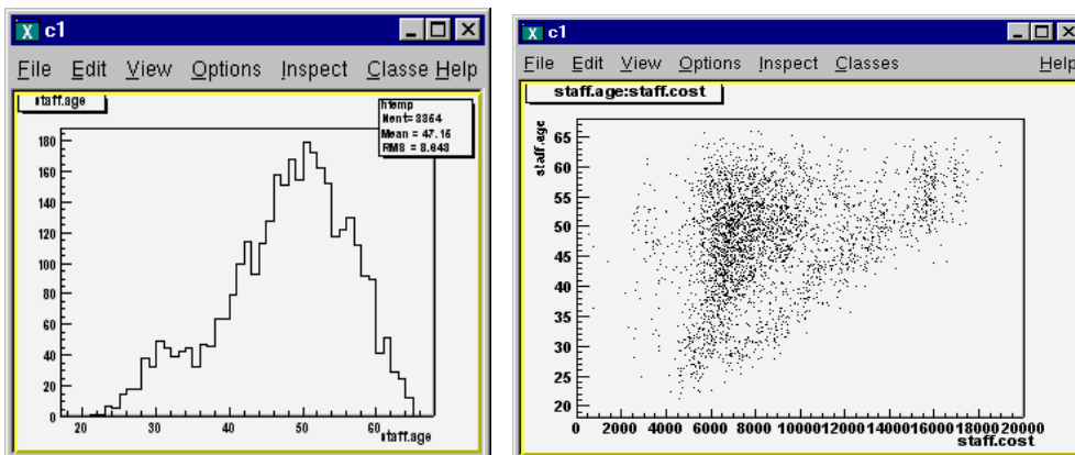
Figure 12-3 A couple of graphs
