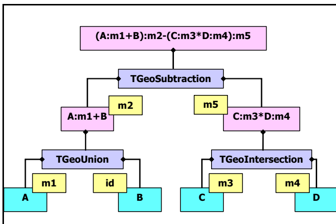
Figure 19-24 Internal representation for composite shapes
