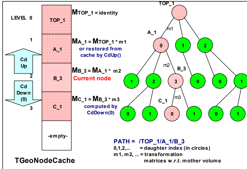
Figure 19-35 Navigation in the geometry hierarchy
