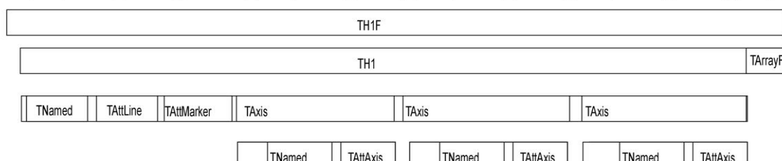
Figure 11-5 A diagram of a streamed TH1F in the buffer
