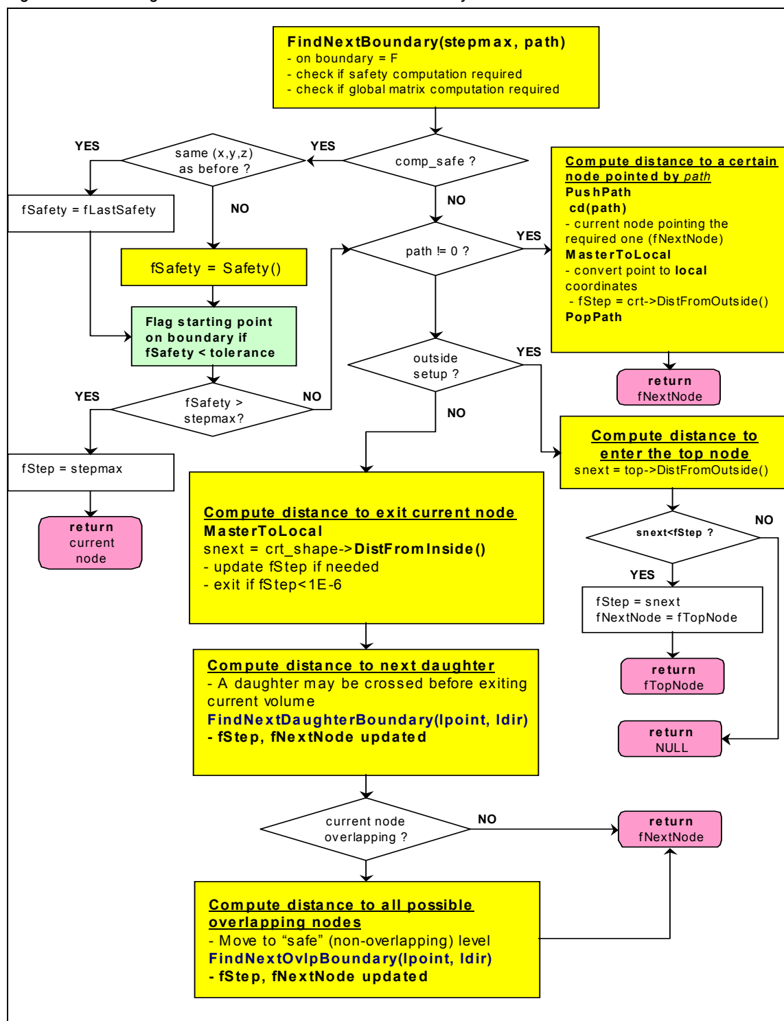
Figure 19-37 Finding the distance to the next crossed boundary
