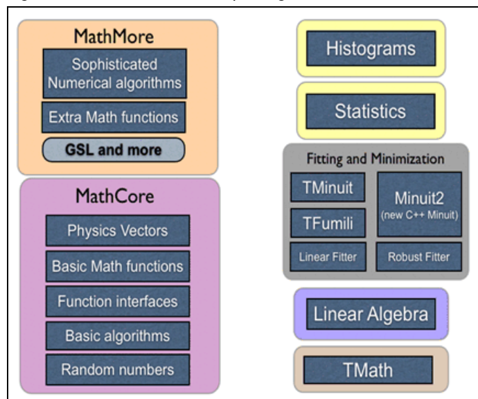
Figure 13-1 Math libraries and packages
