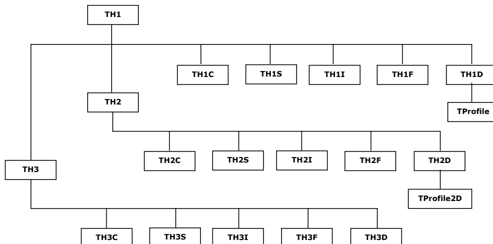
Figure 3-1 The class hierarchy of histogram classes
