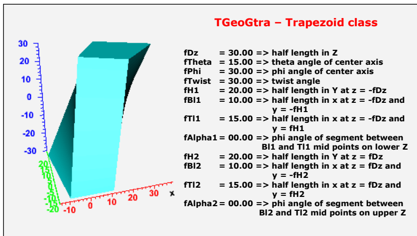
Figure 19-7 TGeoGtra class
