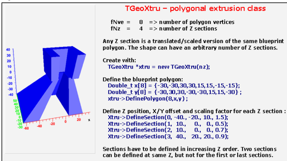
Figure 19-21 TGeoXtru Class
