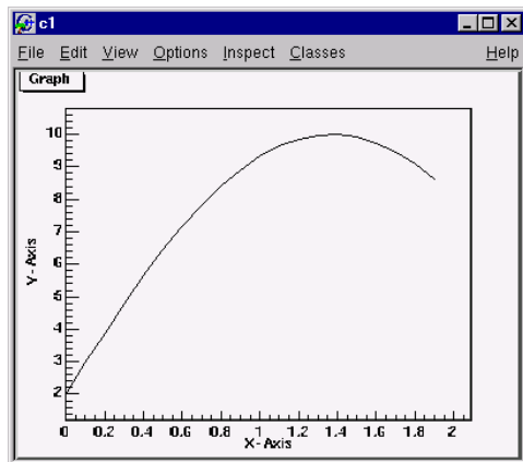
Figure 4-16 A graph with axis titles
