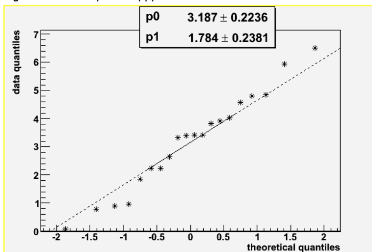
Figure 4-11 Examples of qq-plots of 1 dataset
