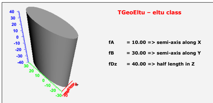
Figure 19-12 TGeoEltu Class
