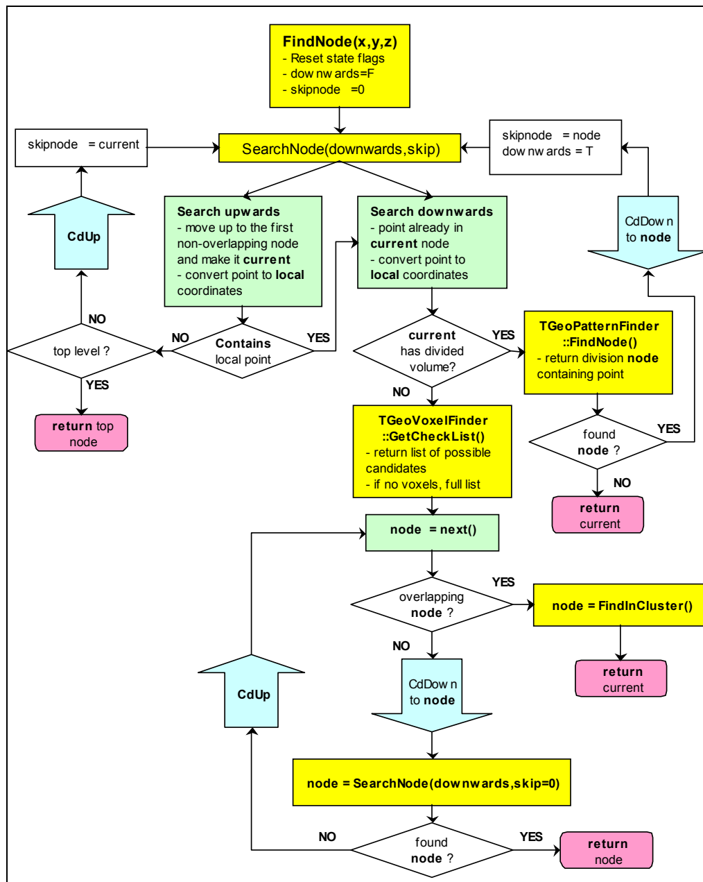
Figure 19-36 Finding the location of a point in the geometry hierarchy
