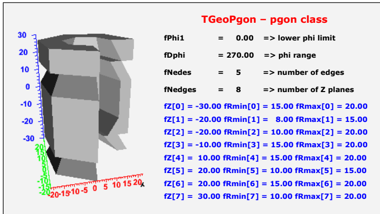
Figure 19-20 TGeoPgon Class
