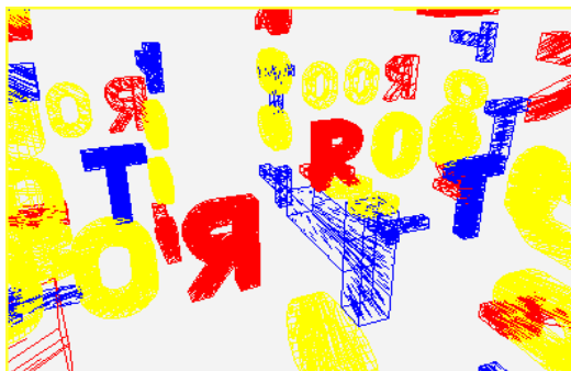
Figure 19-32 Random rays
