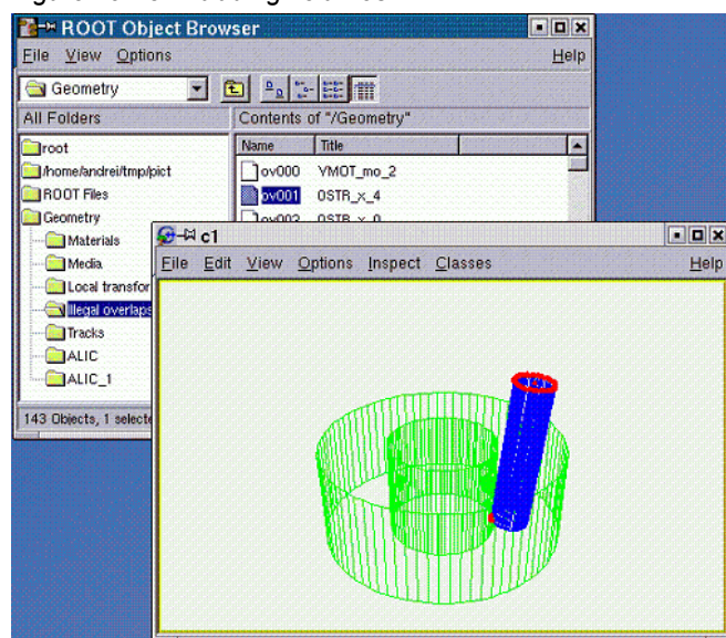
Figure 19-28 Extruding volumes
