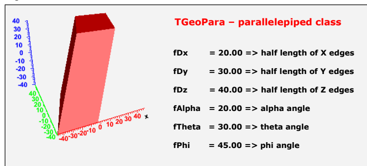
Figure 19-3 TGeoPara class
