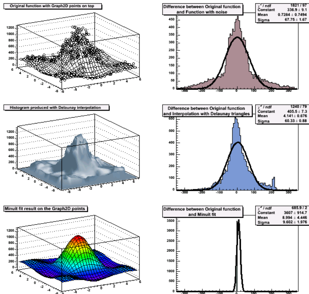
Figure 4-15 Output of macro graph2dfit.C
