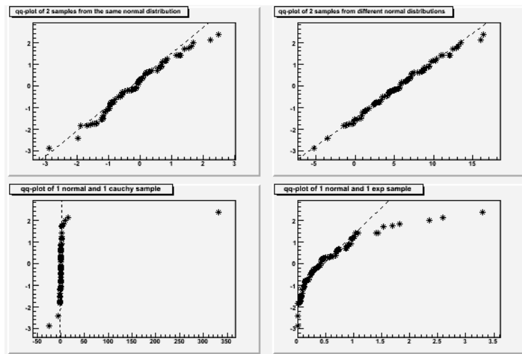
Figure 4-10 Examples of qq-plots of 2 datasets
