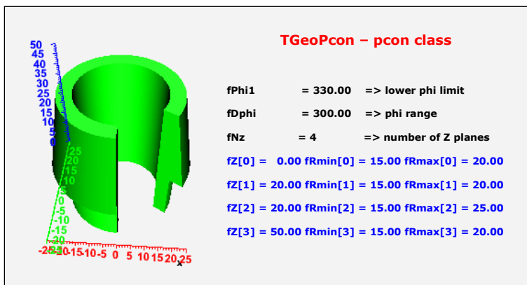
Figure 19-19 TGeoPcon Class
