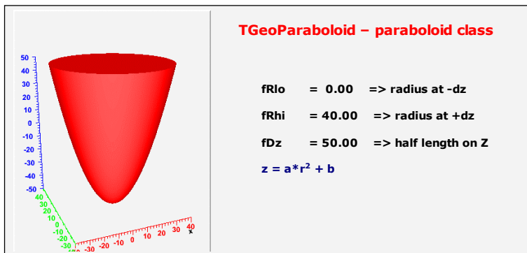
Figure 19-18 TGeoParaboloid Class
