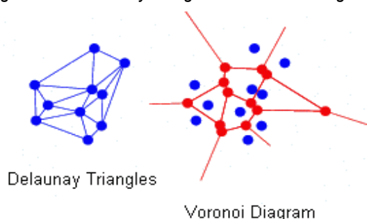
Figure 4-13 Delaunay triangles and Voronoi diagram
