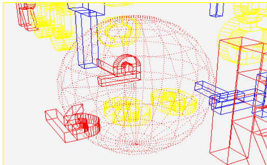
Figure 19-31 Random points
