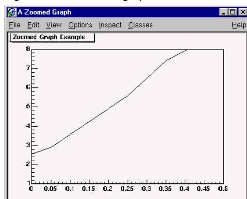
Figure 4-17 A zoomed graph
