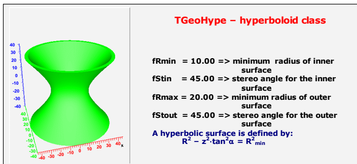
Figure 19-13 TGeoHype Class
