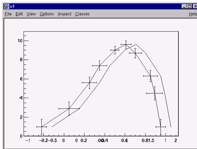
Figure 4-12 A multigraph example
