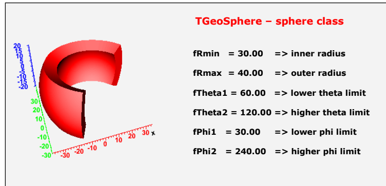
Figure 19-16 TGeoSphere Class
