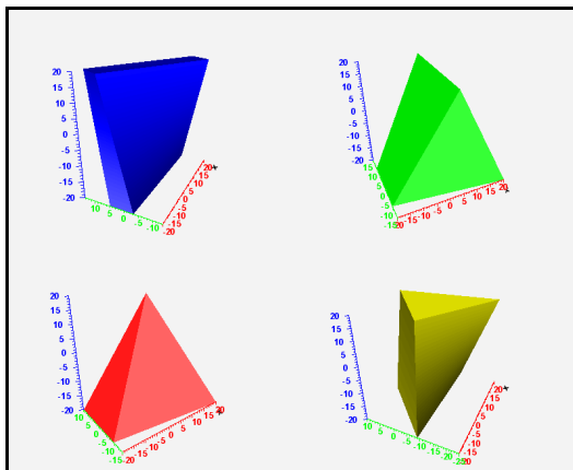
Figure 19-8 TGeoArb8 class
