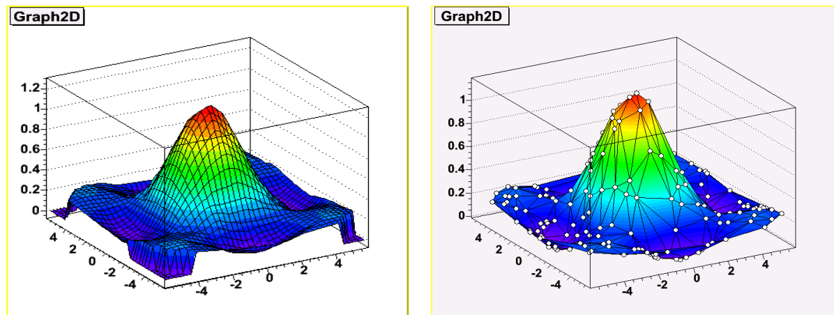
Figure 4-14 Graph2D drawn with option "surf" and "tril p0"
