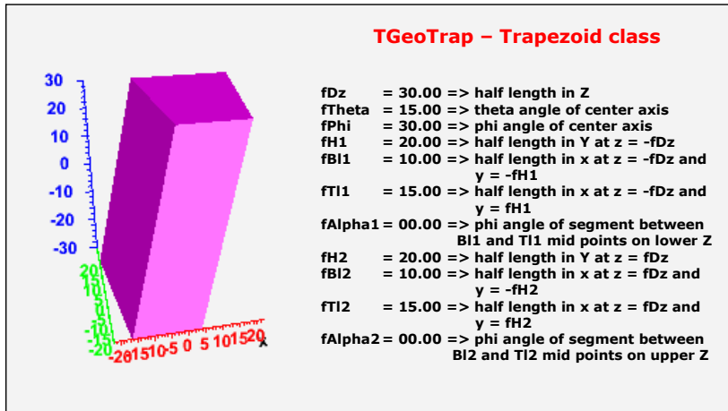
Figure 19-6 TGeoTrap Class
